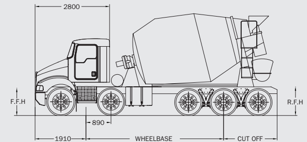
DAY CAB
