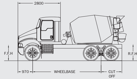
DAY CAB
